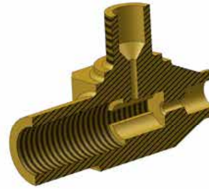
SECTION 3-2 SCALE 1:1
